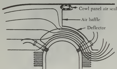
FIGURE 6-44. Cylinder head baffle and deflector system.
